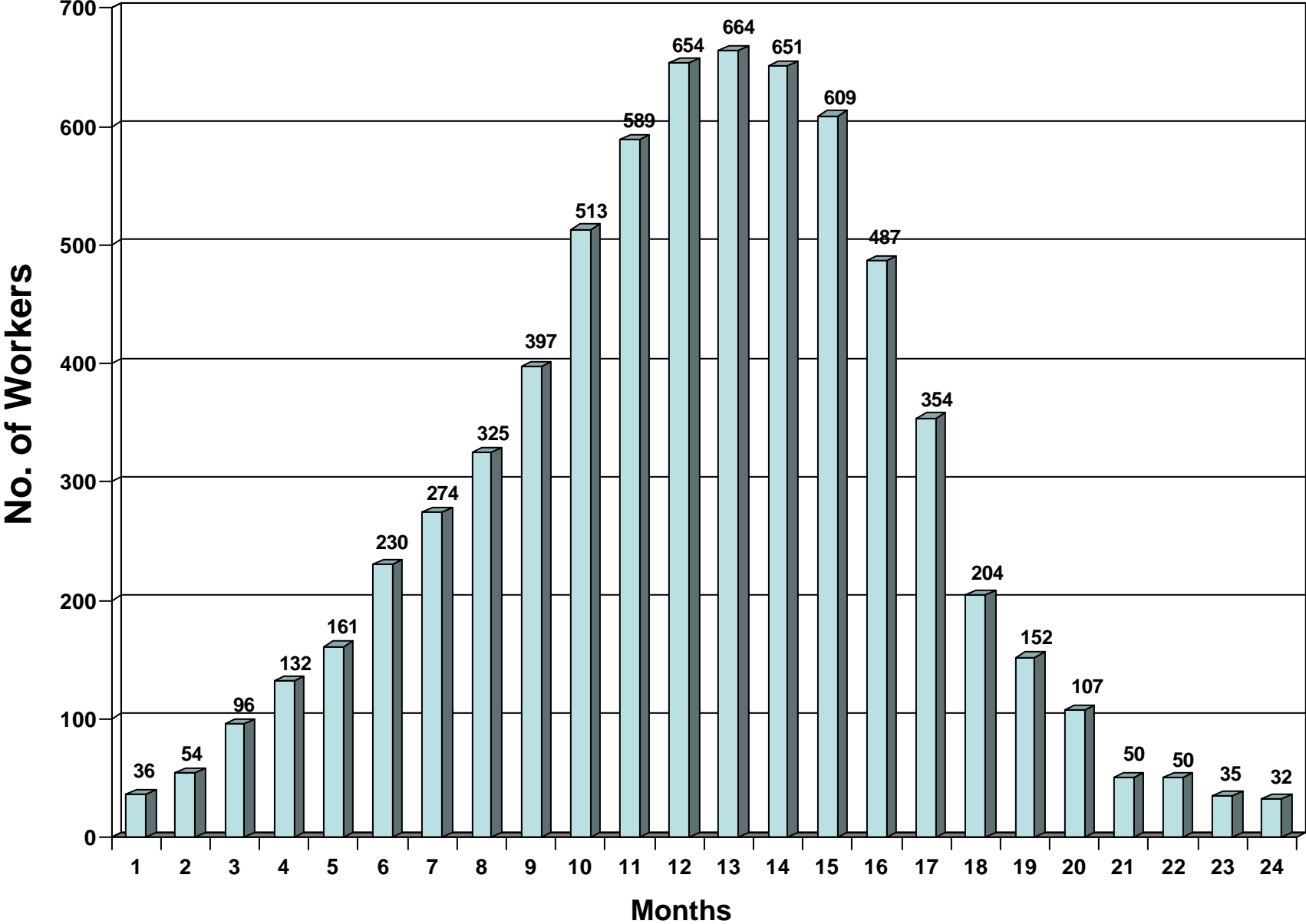
FIGURE 7-1 Estimated Construction Manpower By Month
