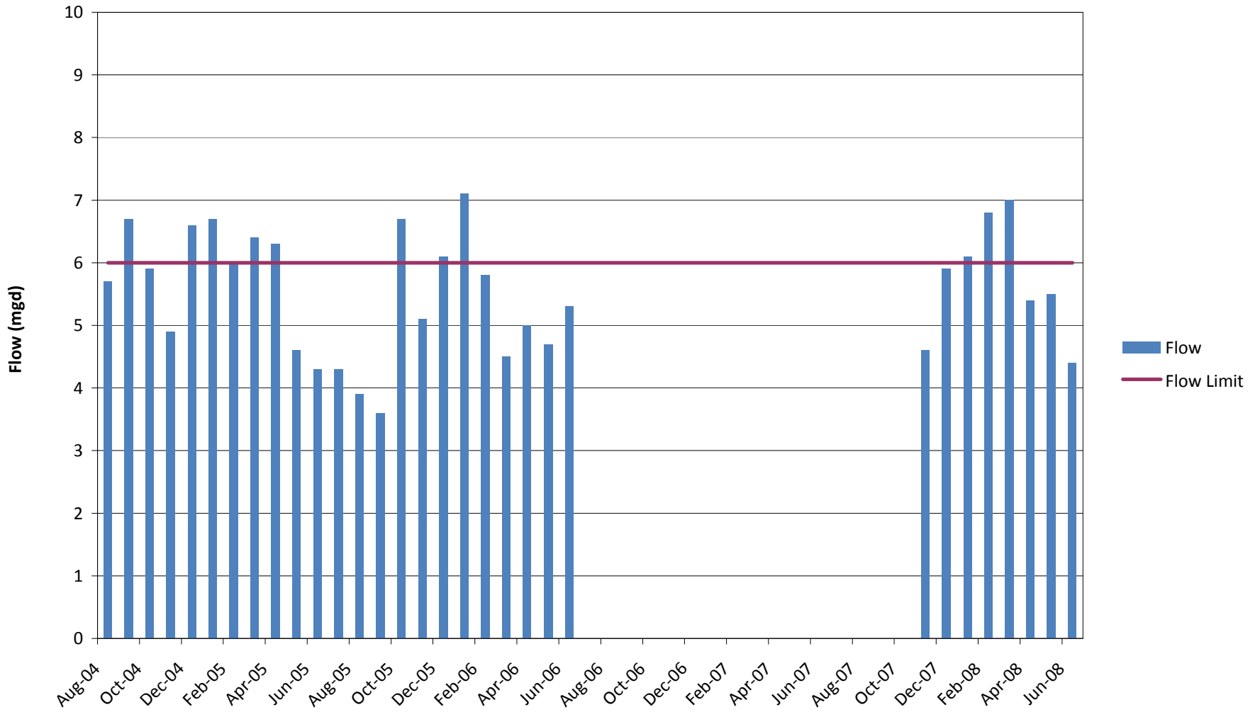
Figure 21 Middletown STP Average Monthly Flow
