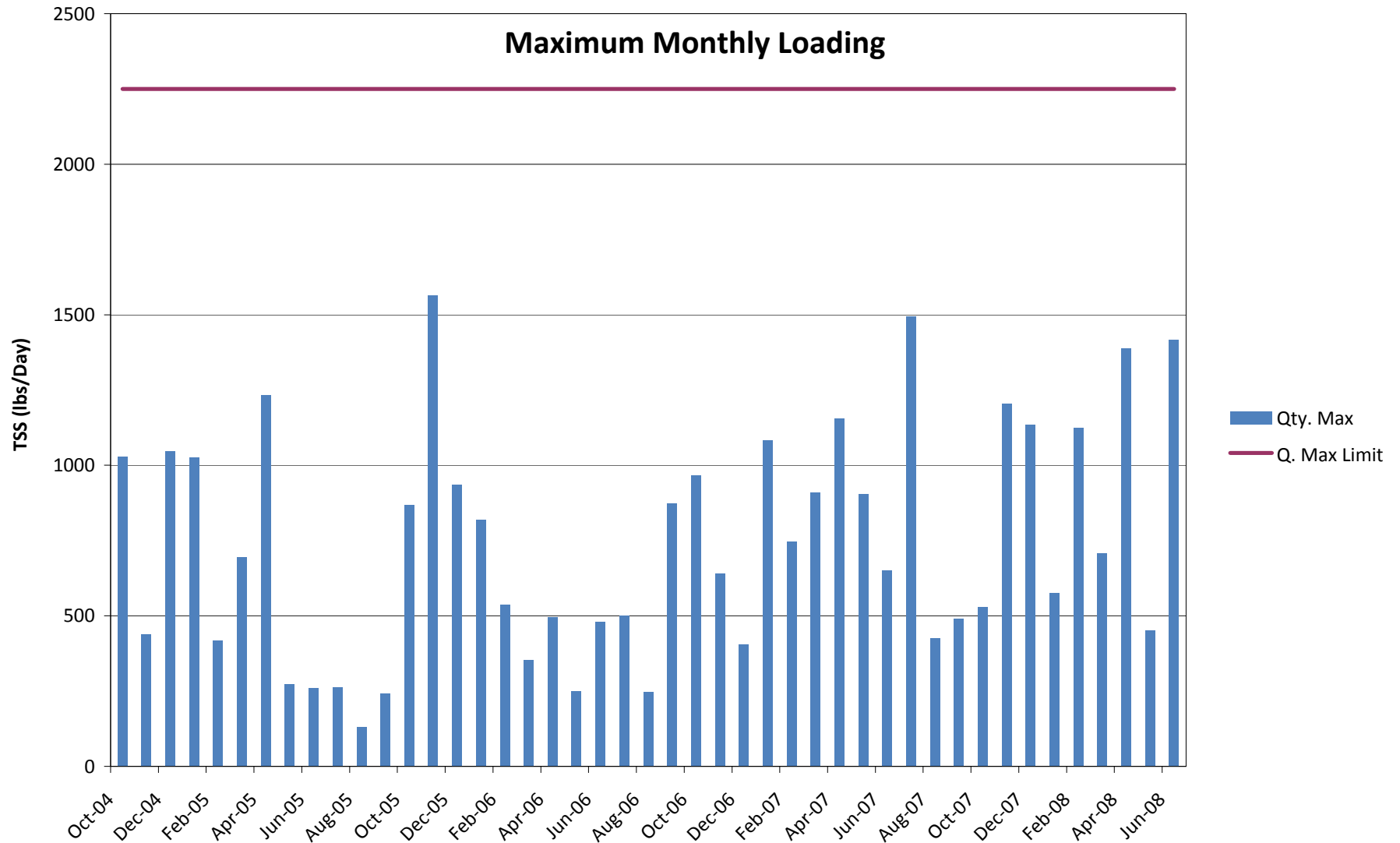
Figure 7 Middletown STP Total Suspended Solids (TSS)
