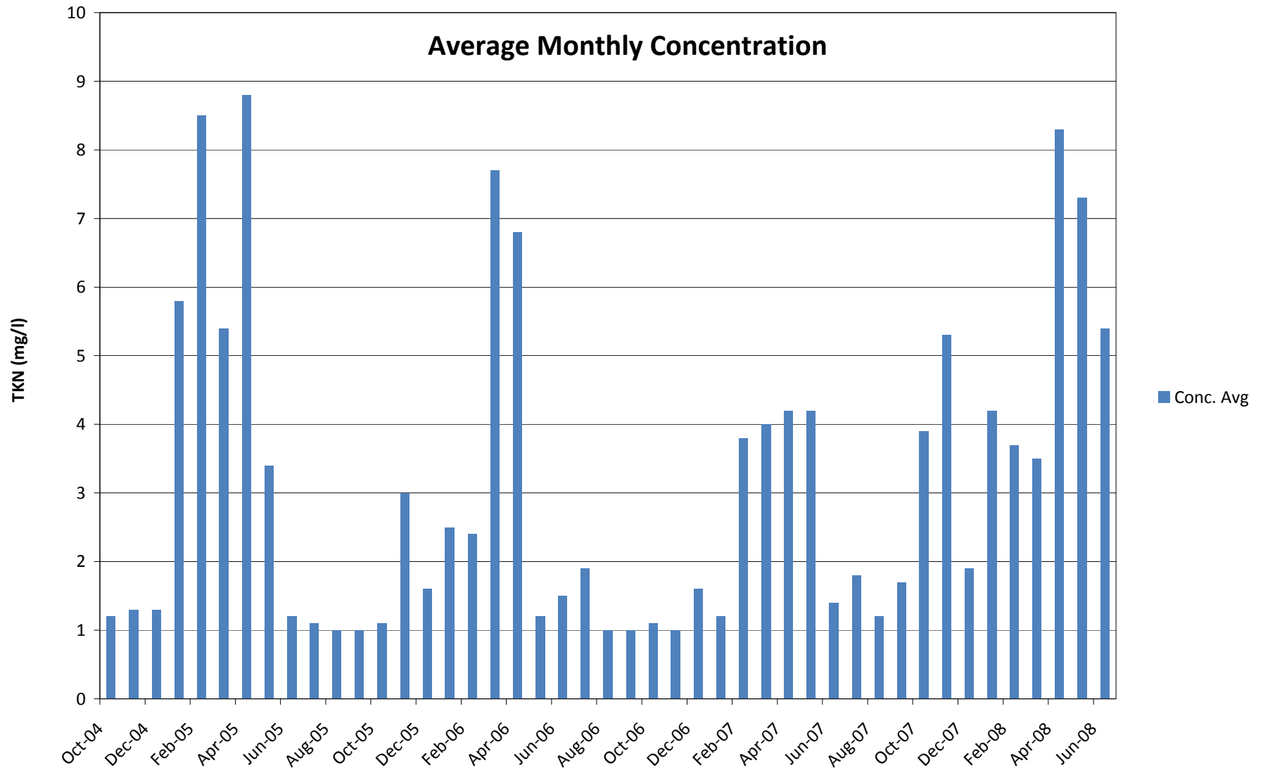
Figure 14 Middletown STP Total Kjeldahl Nitrogen (as N) (TKN)
