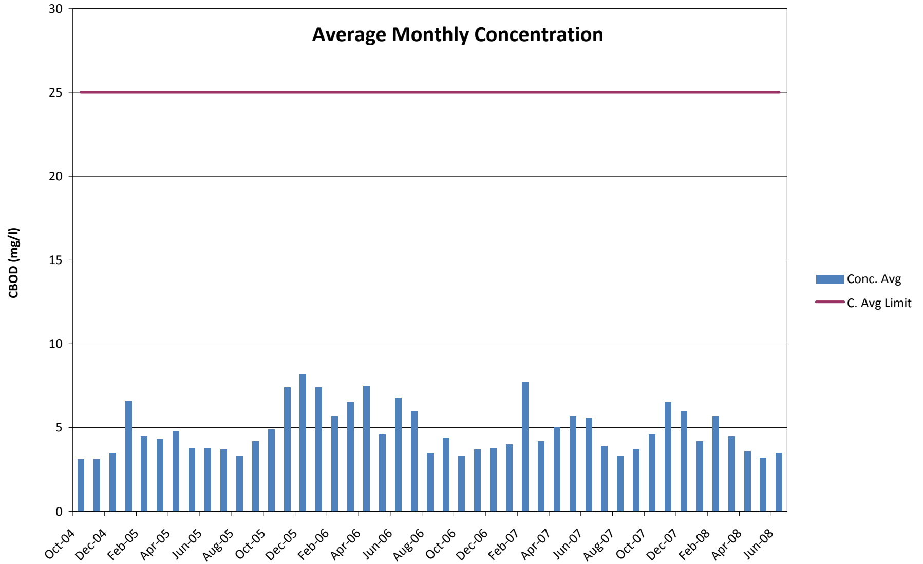
Figure 2 Middletown STP Carbonaceous Biochemical Oxygen Demand (CBOD)
