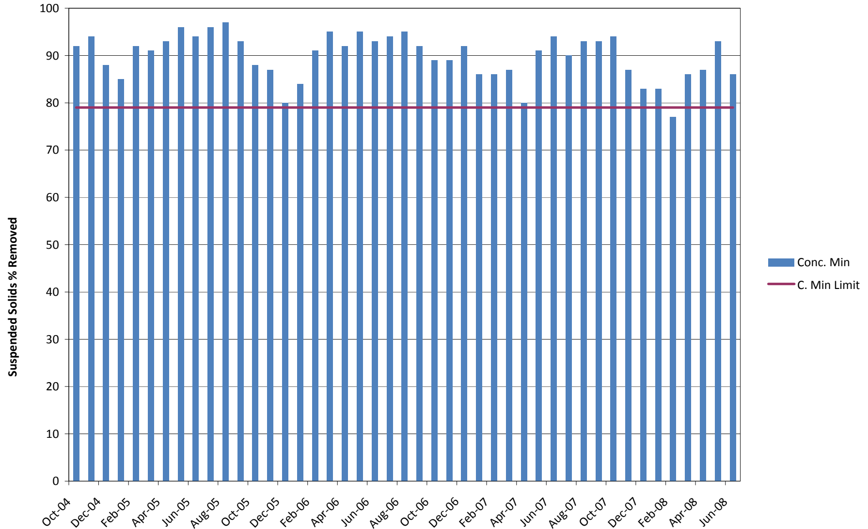
Figure 9 Middletown STP Suspended Solids Percent (%) Removal
