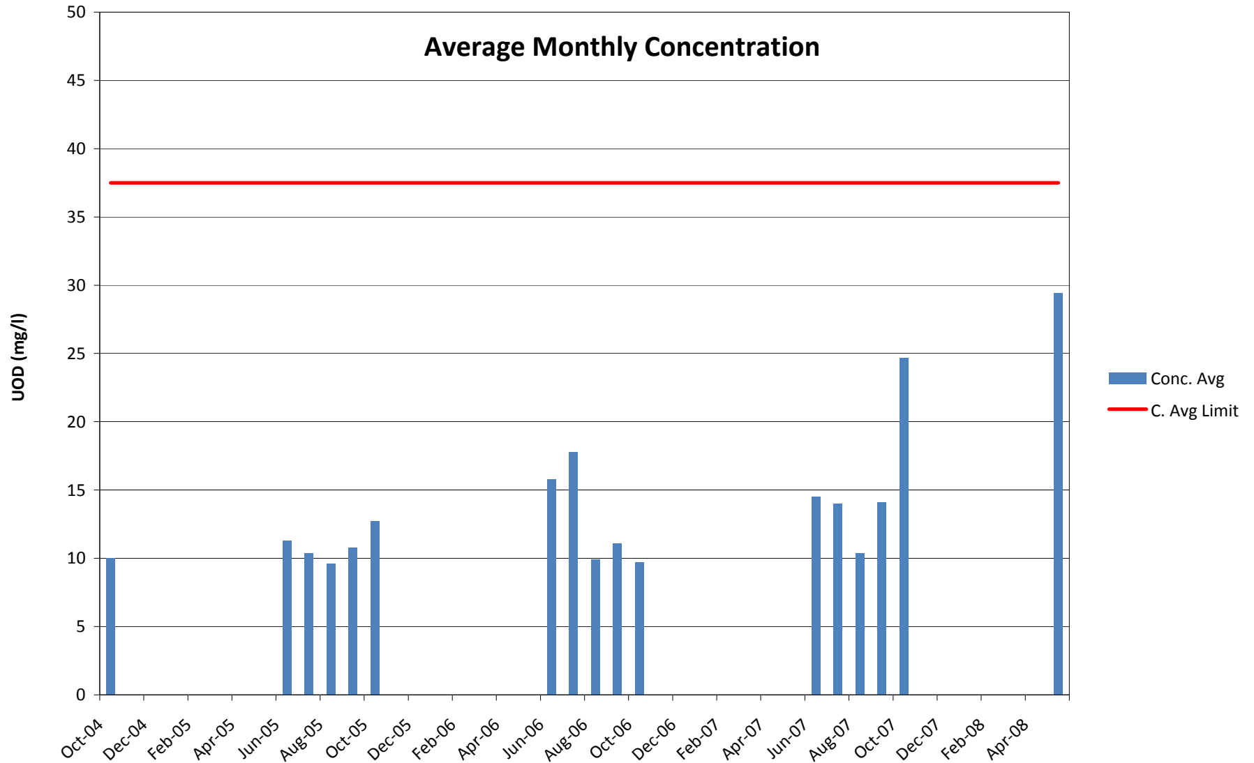
Figure 11 Middletown STP Ultimate Oxygen Demand (UOD)
