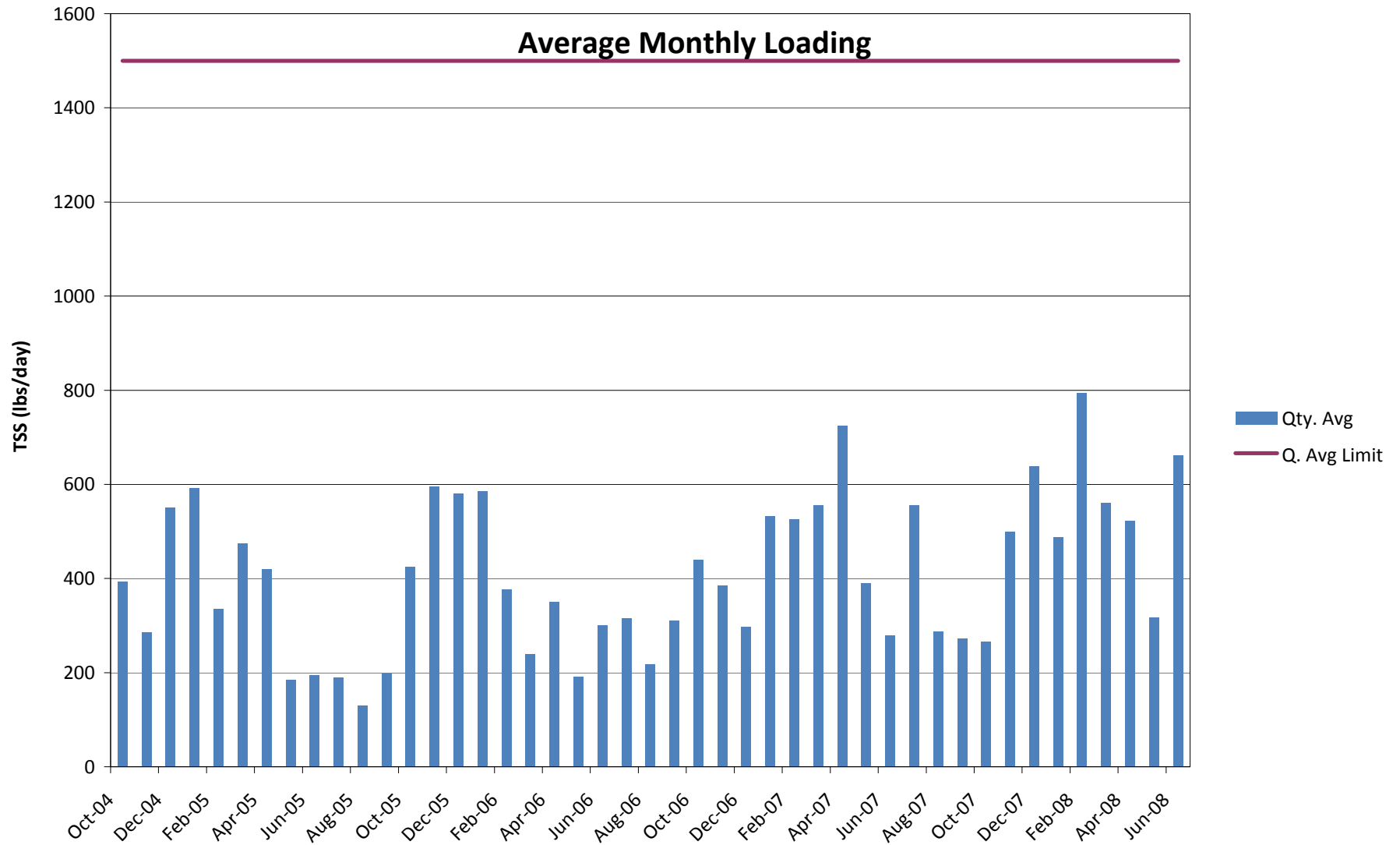
Figure 8 Middletown STP Total Suspended Solids (TSS)
