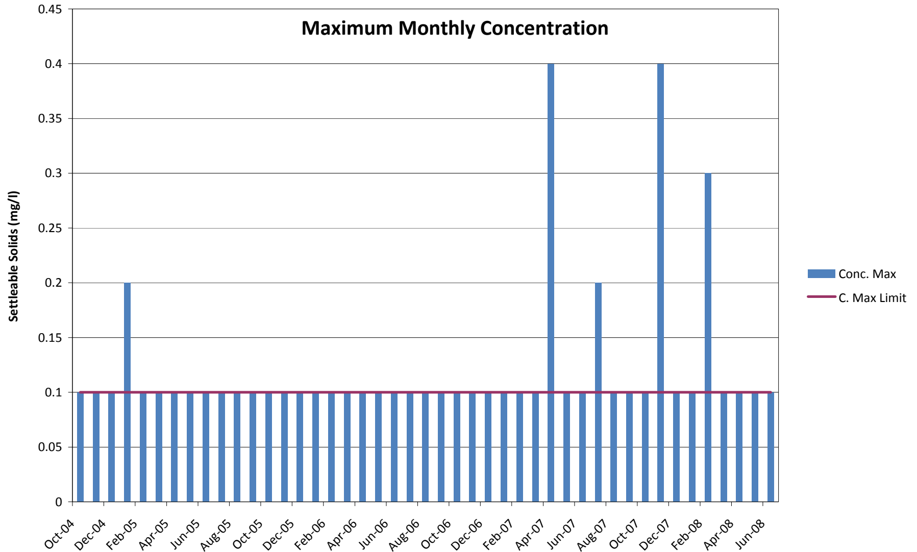
Figure 10 Middletown STP Settleable Solids
