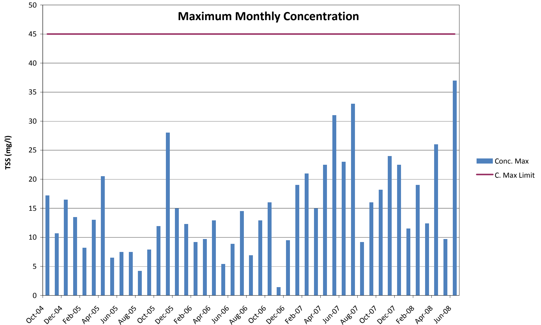
Figure 5 Middletown STP Total Suspended Solids (TSS)
