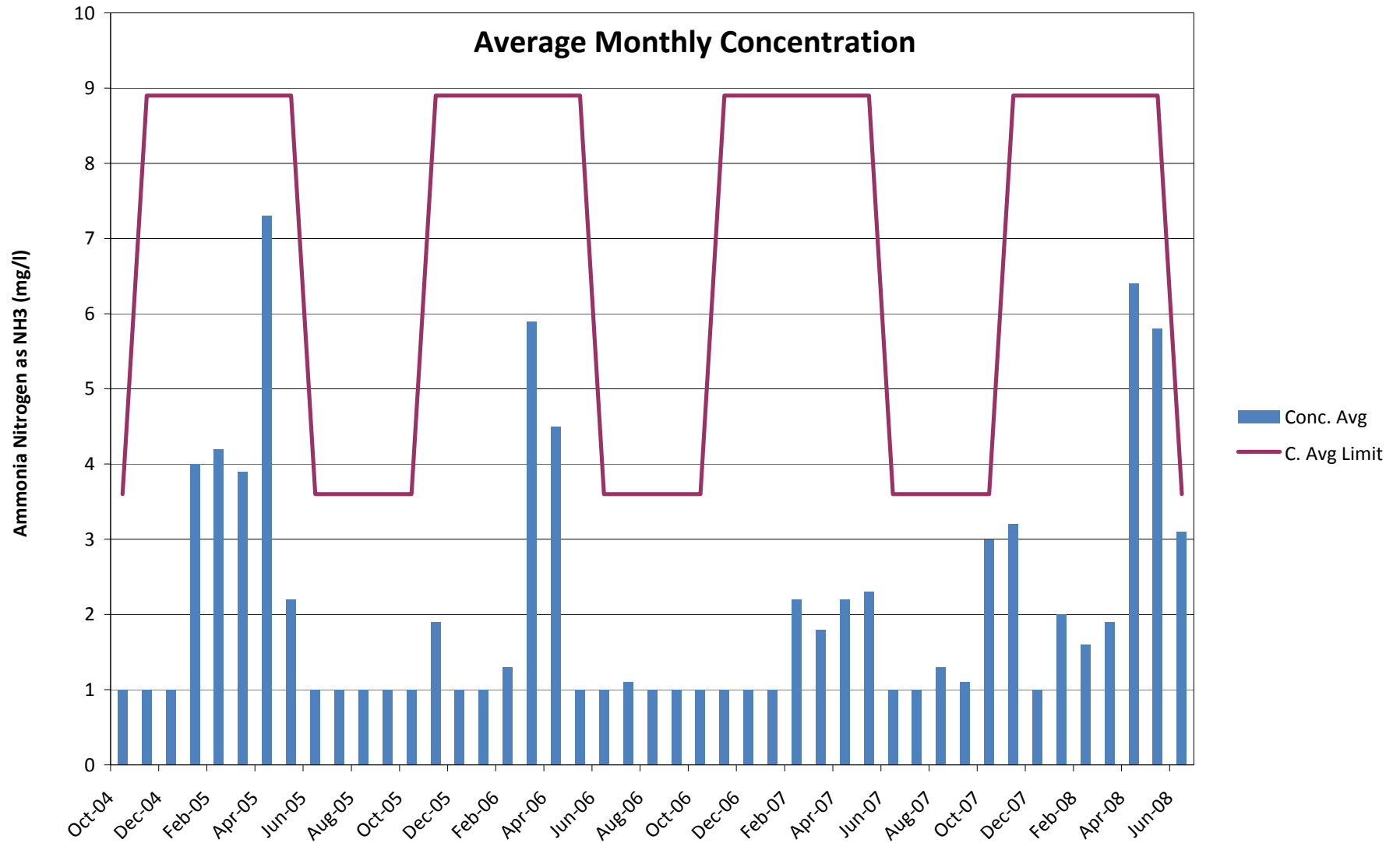
Figure 13 Middletown STP Ammonia Nitrogen (as NH 3 )
