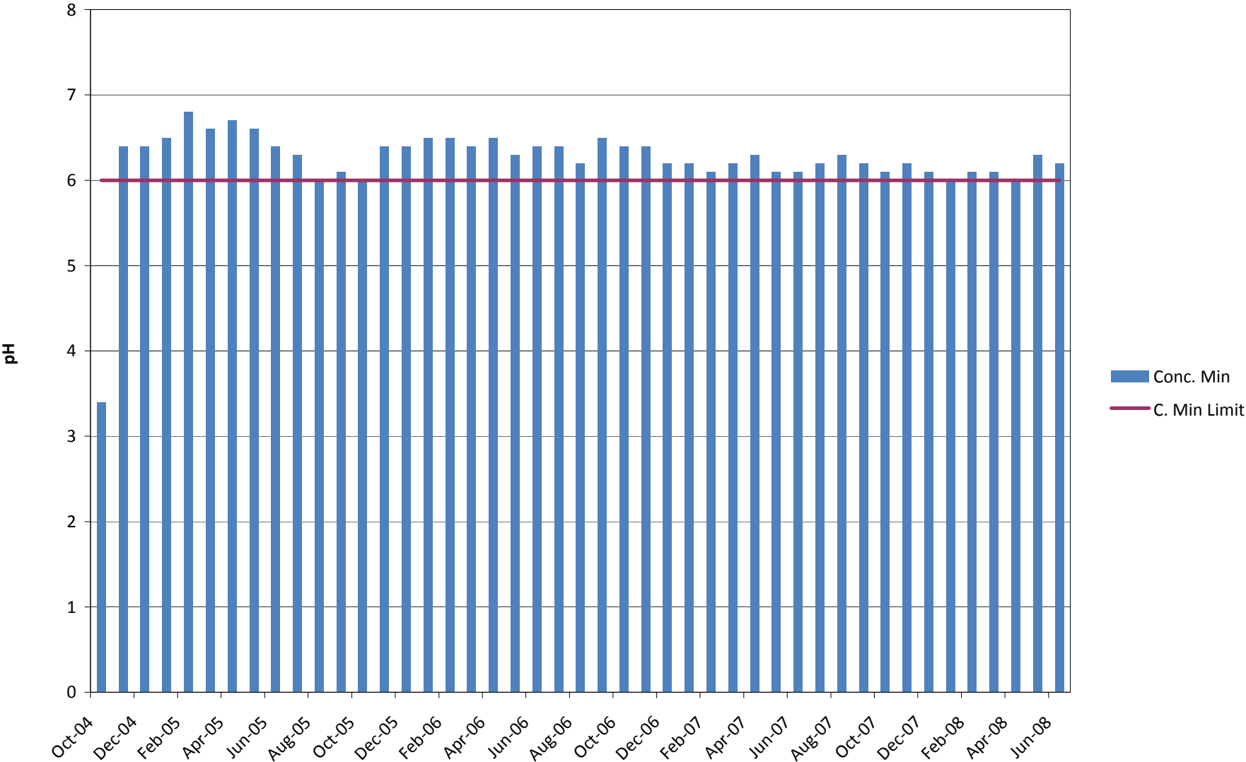
Figure 16 Middletown STP Minimum pH
