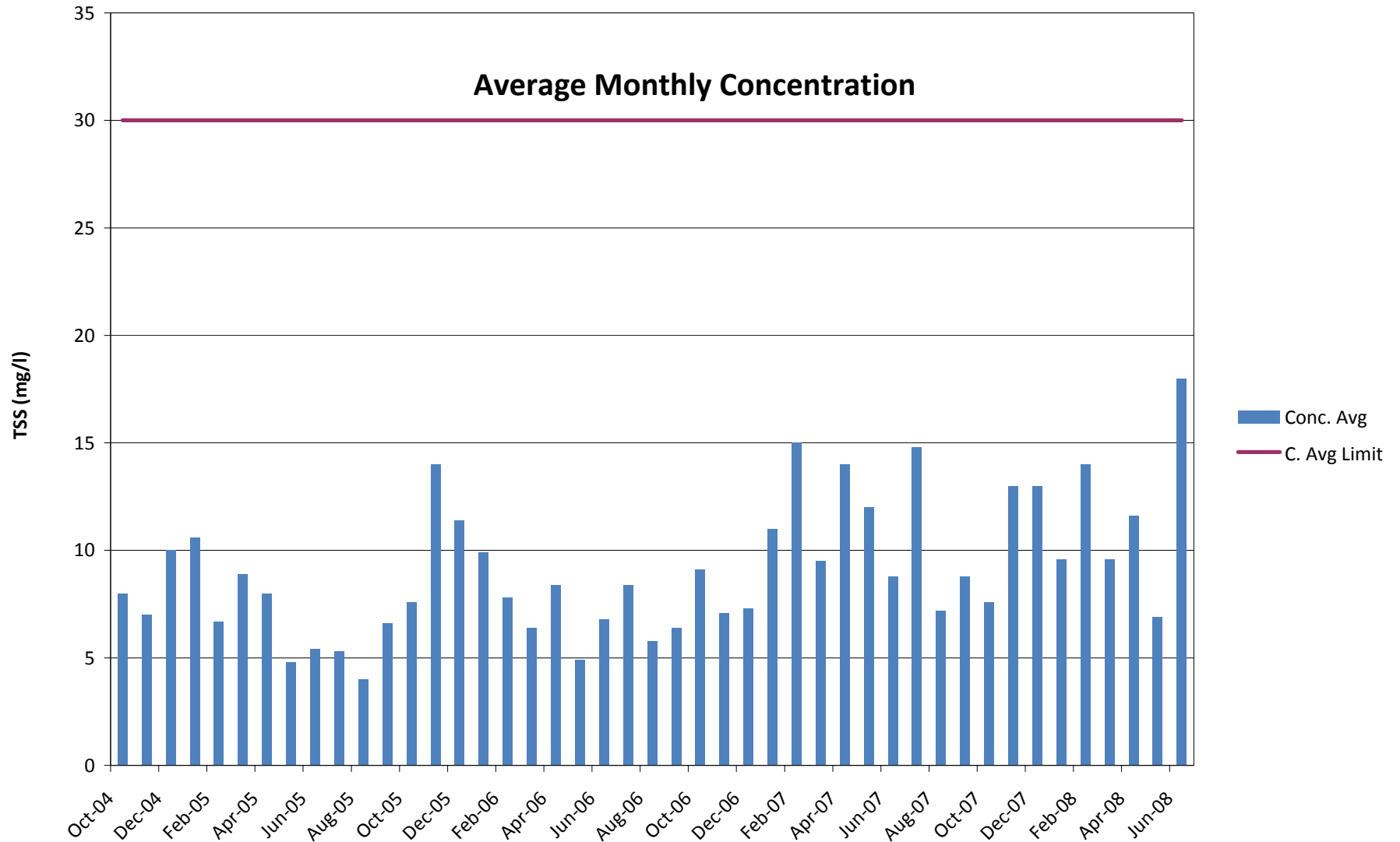
Figure 6 Middletown STP Total Suspended Solids (TSS)
