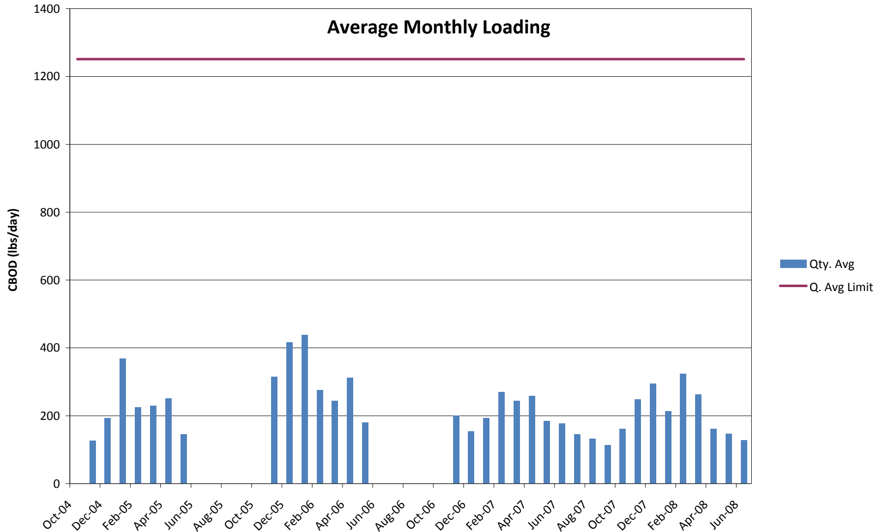
Figure 4 Middletown STP Carbonaceous Biochemical Oxygen Demand (CBOD)
