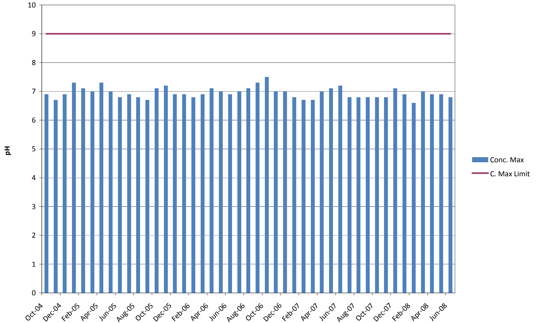
Figure 17 Middletown STP Maximum pH
