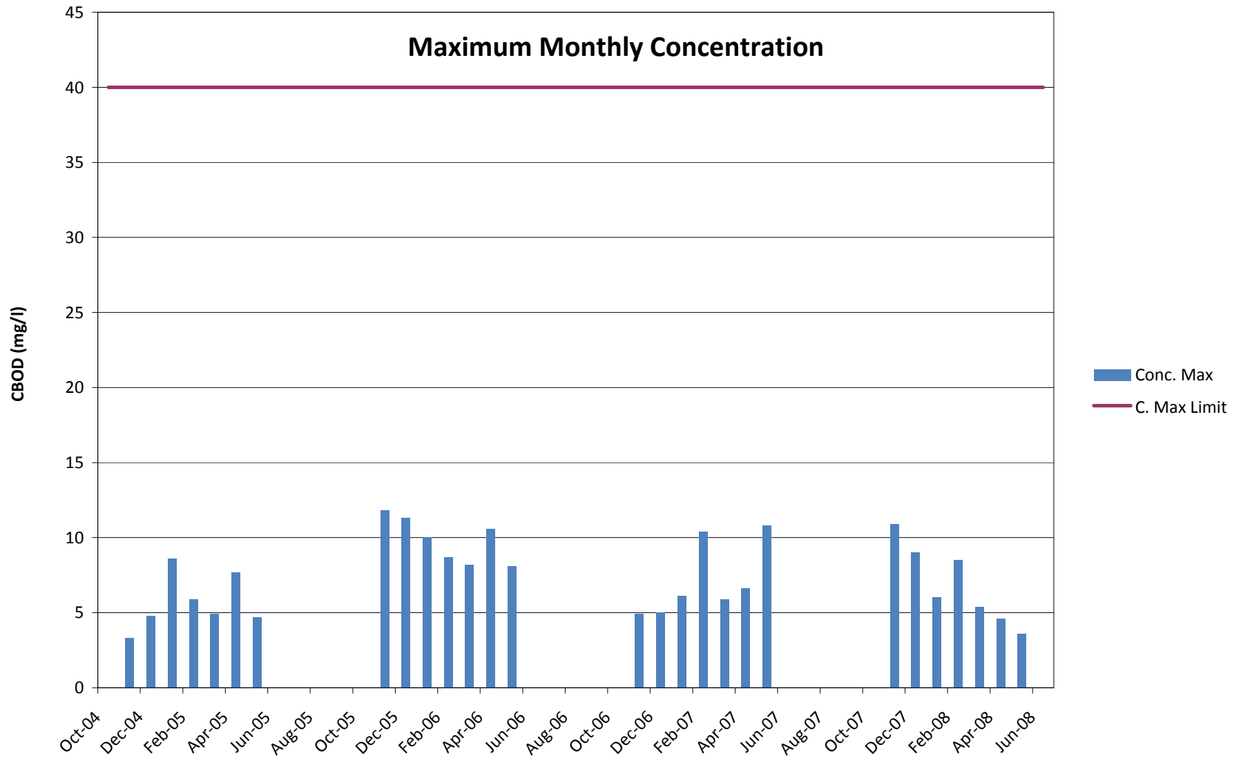
Figure 1 Middletown STP Carbonaceous Biochemical Oxygen Demand (CBOD)
