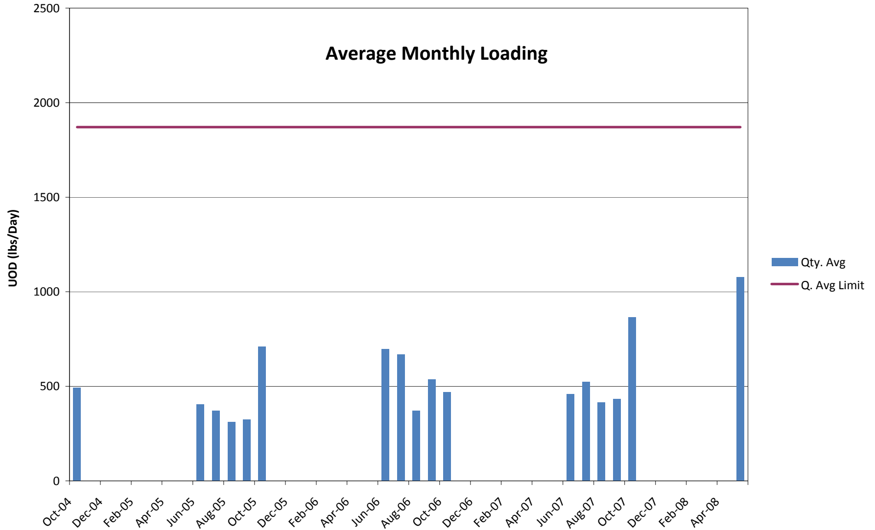
Figure 12 Middletown STP Ultimate Oxygen Demand (UOD)
