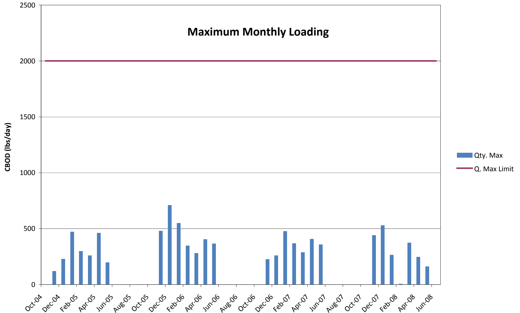
Figure 3 Middletown STP Carbonaceous Biochemical Oxygen Demand (CBOD)
